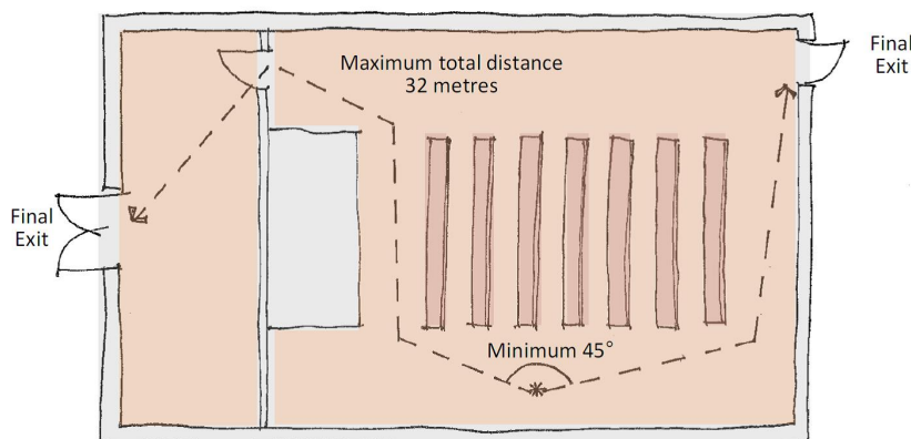
For 61 to 600 persons there must be two final exits
