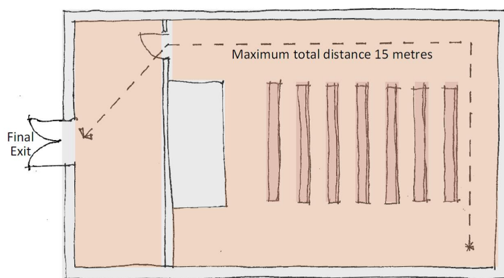
With one final exit for a room for up to 60 persons
